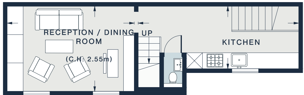
FIRST FLOOR
