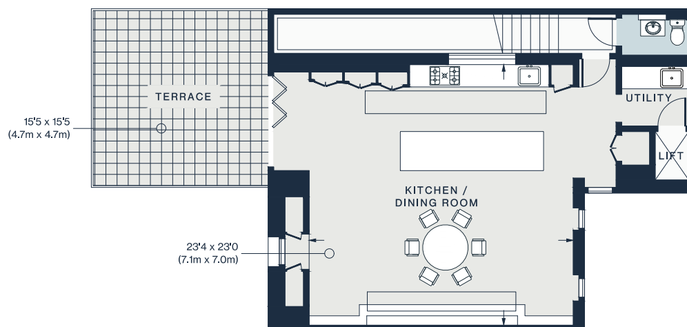
SECOND FLOOR
