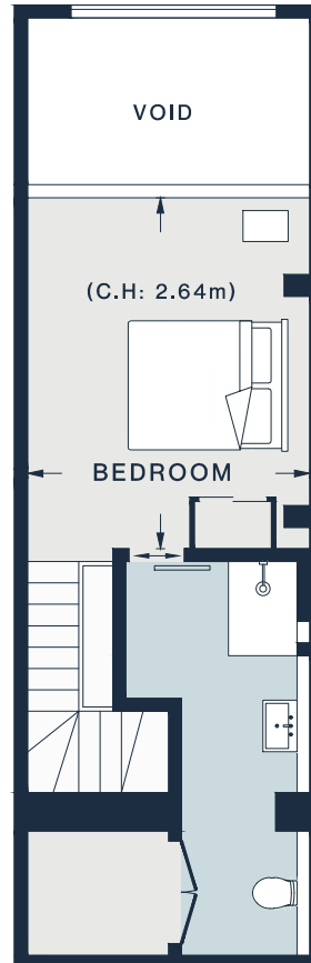
FIRST FLOOR (MEZZANINE)
