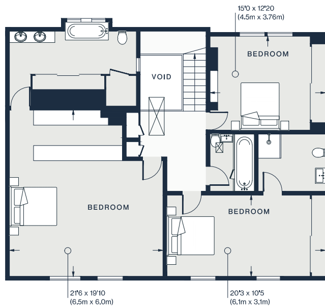
FOURTH FLOOR
