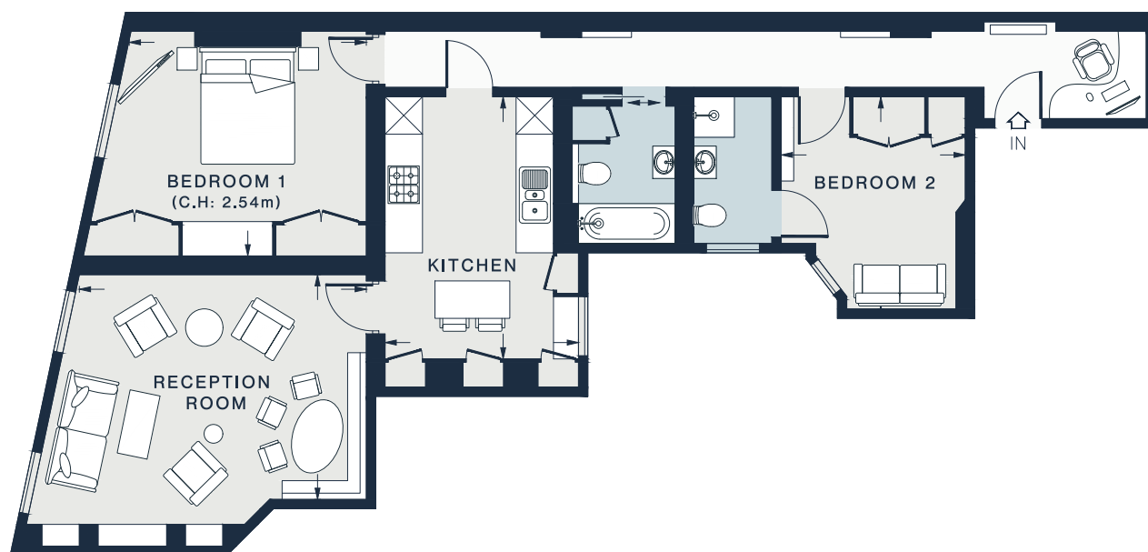
FOURTH FLOOR
