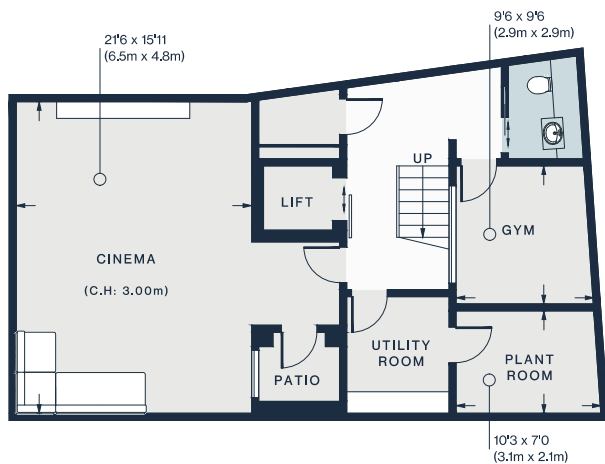
BASEMENT
